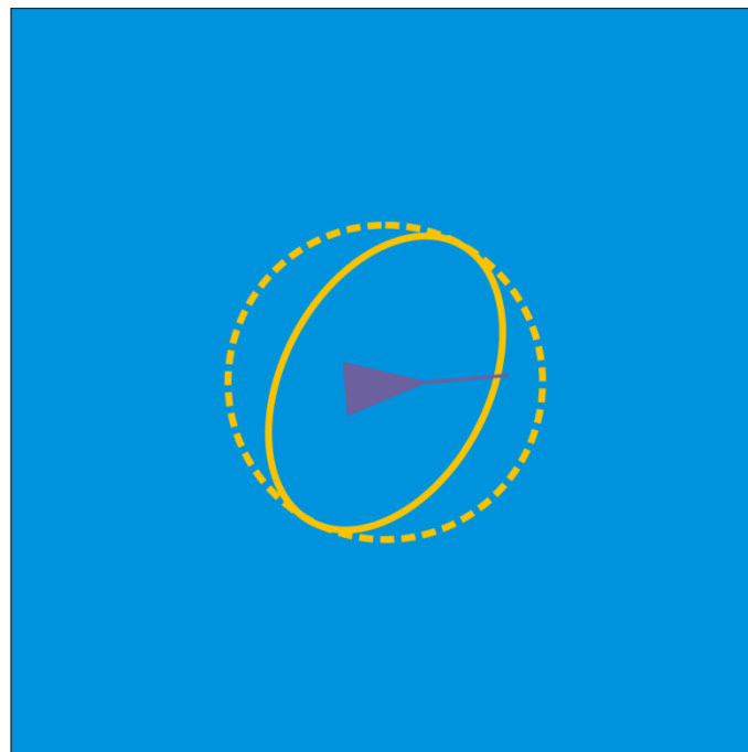
Figure 3.7 – Horizontal Protection Level (yellow ellipse) has reached the level of the Horizontal Alert Limit (yellow dashed circle). This configuration indicates estimated positioning accuracy performance is becoming poor but is still at the HAL level; HPL = HAL .
