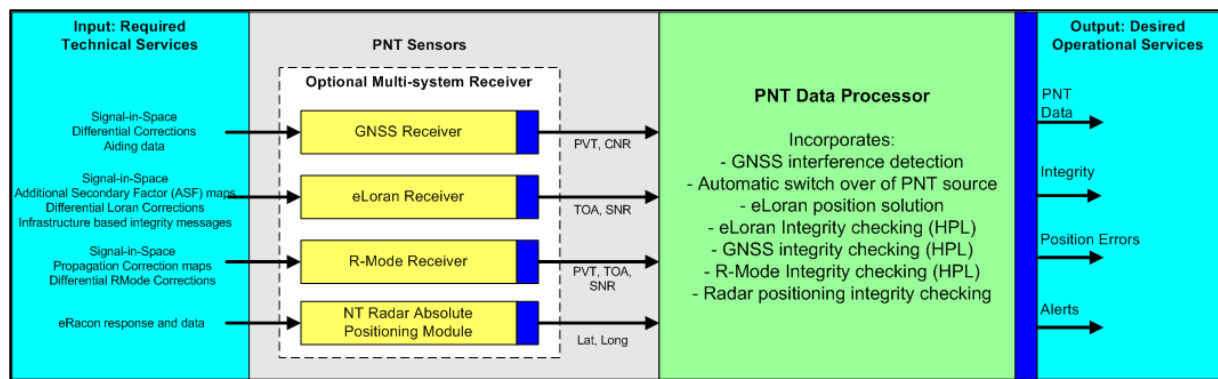
Figure 2.3 – Structure of the ACCSEAS ship-side Multi Source Positioning Service architecture.
