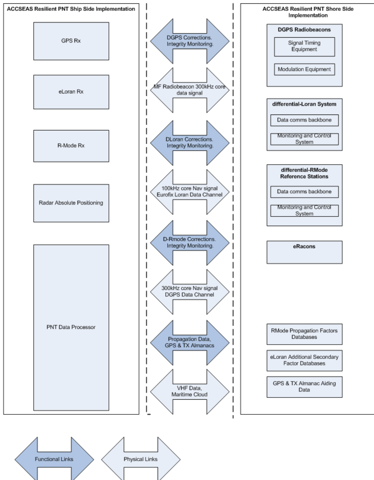
Figure 3.2 – Organisation of ship-side and shore-side components of the Resilient PNT system with Functional and Physical Data Links.
