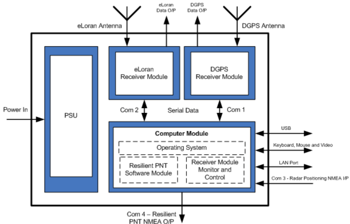
Figure 5.1 – Schematic of the ACCSEAS MSPS receiver and its internal components.
