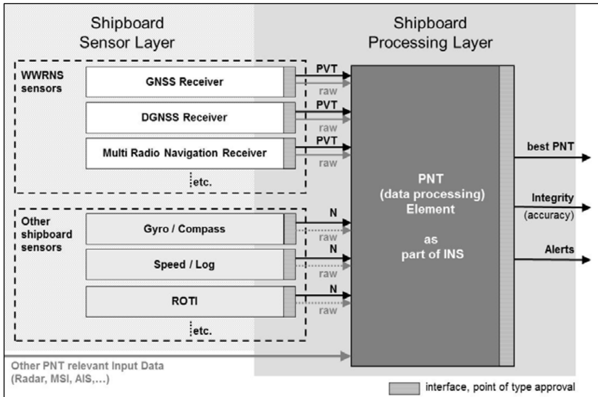
Figure 2.2 – Ship-side PNT entity with PNT Data Processing Element.
