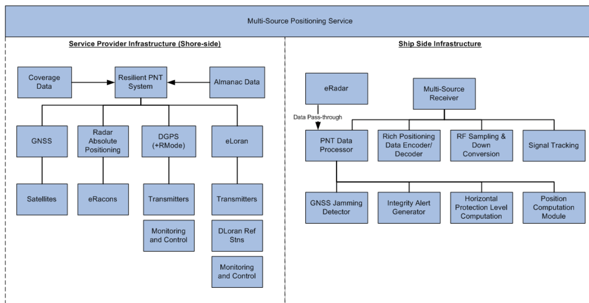
Figure 3.1 – Top down design of Multi-Source Positioning Service. (Note that radar absolute positioning, although demonstrated, will not be implemented within the timeframe of ACCSEAS).
