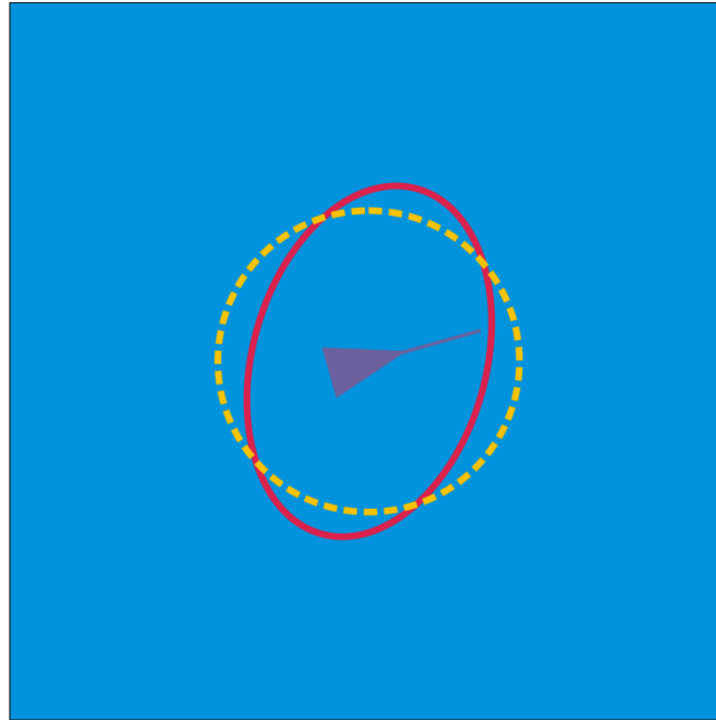
Figure 3.6 – Horizontal Protection Level (red ellipse) has breached the Horizontal Alert Limit (yellow dashed circle). This configuration indicates positioning accuracy performance is predicted to be bad and cannot be relied upon; HPL > HAL .
