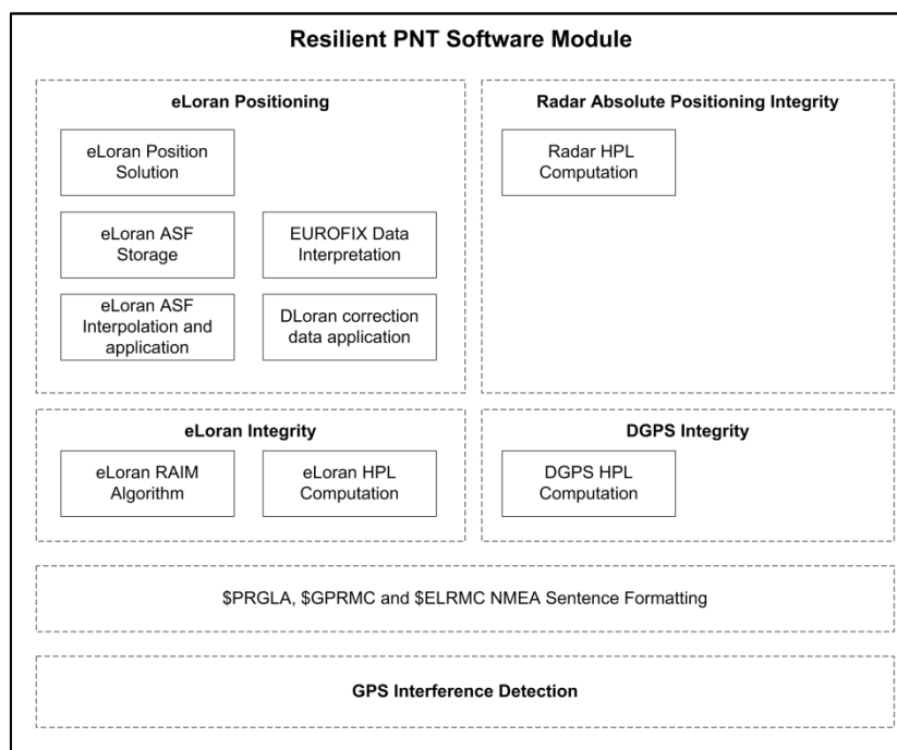
Figure 3.3 – The main functions of the ACCSEAS Resilient PNT Data Processor. (Note that the HPL computation for radar will not be implemented under ACCSEAS.)
