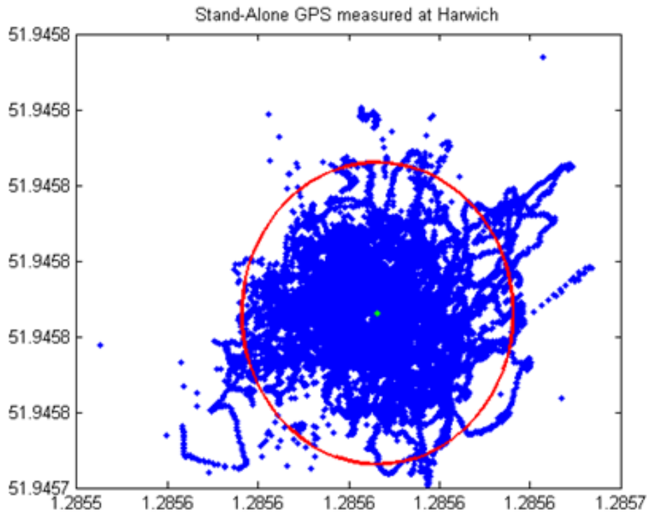
Figure 3.4 – GPS positioning error.
