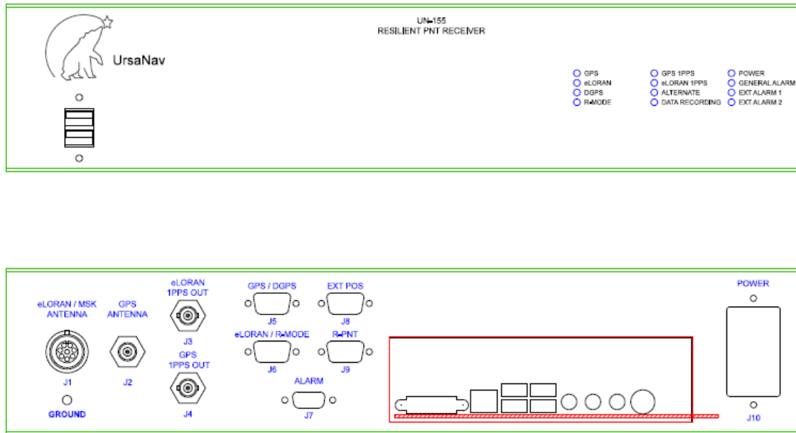
Figure 5.2 – Example layout of ports on the ACCSEAS MSPS receiver.
