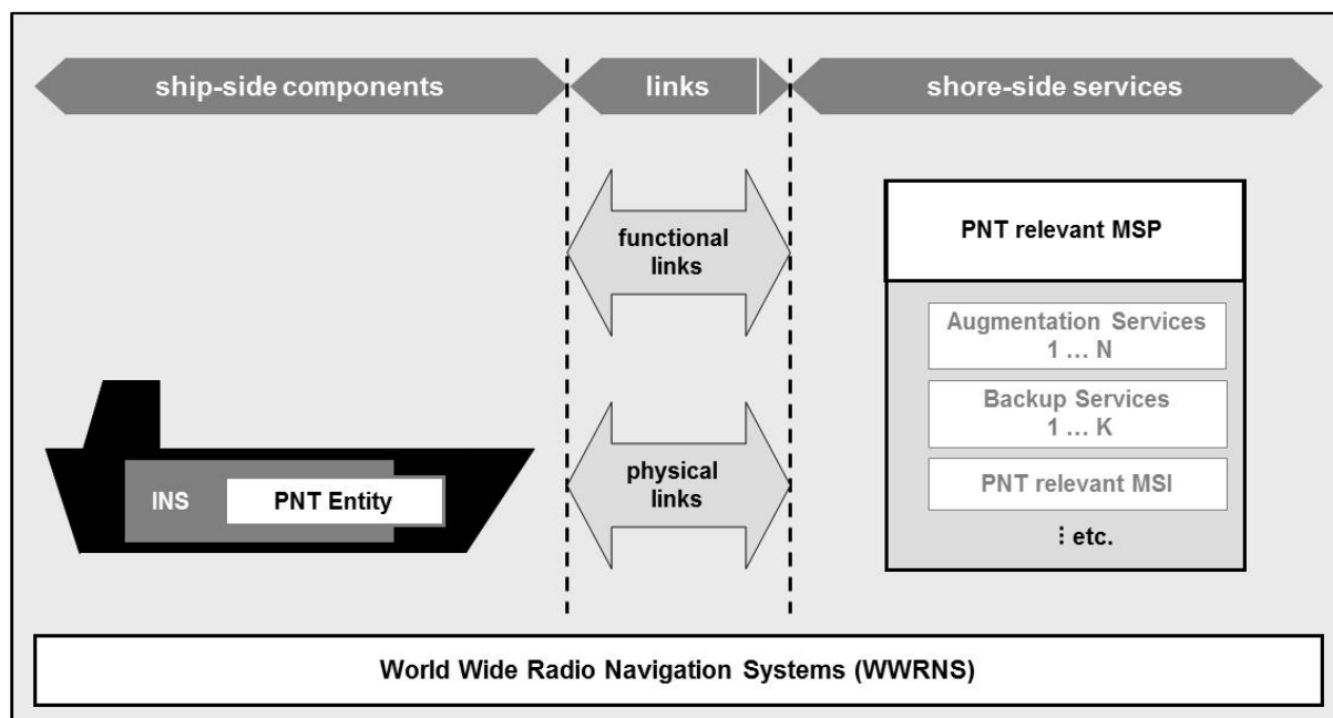
Figure 2.1 - Generic architecture of the maritime Integrated PNT system. After [1].
