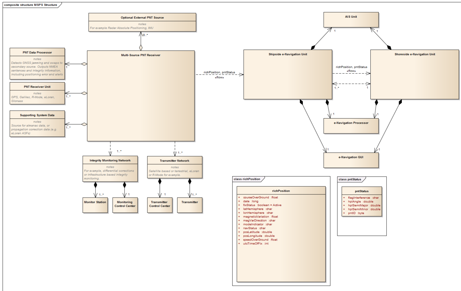
Figure 2.4 – Entity Diagram for Multi-Source Positioning Service. This does not yet consider IHO S-100 data models but is a reference for future development work in this area.
