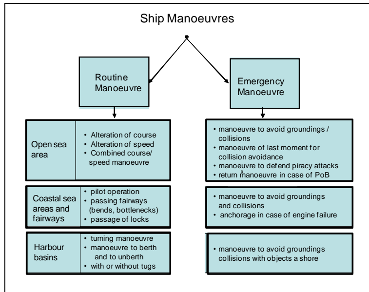
Figure 9: Systematization of ship manoeuvring
