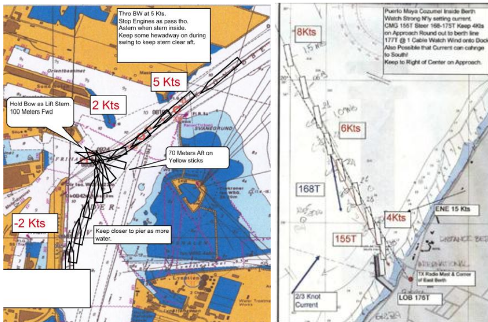
Figure 8: Samples of two plans for berthing a ship in a harbour
