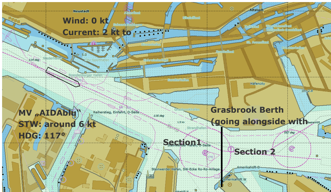
Figure 10: Exercise area and environmental conditions in Port of Hamburg for berthing scenario, divided into two sections for planning the manoeuvres
