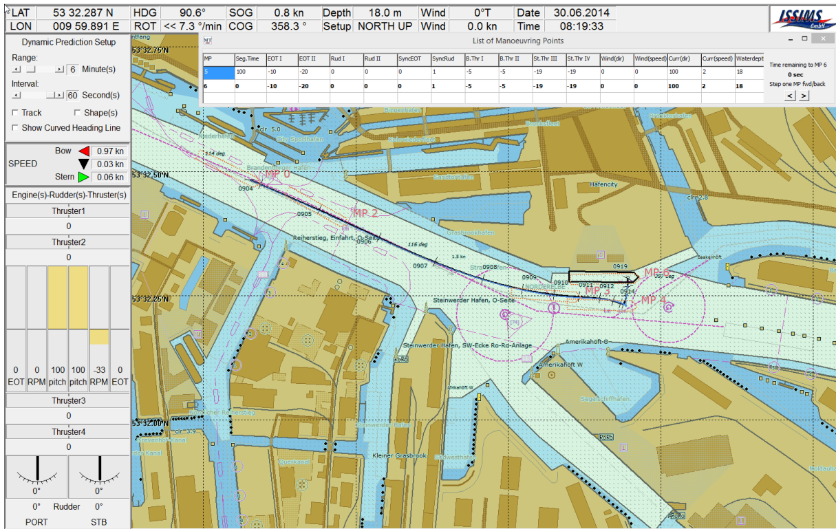
Figure 17: Result of manoeuvring for a trainee with advanced briefing preparation and full support by fast time simulation (Total Manoeuvring Time about 15.5 min)
