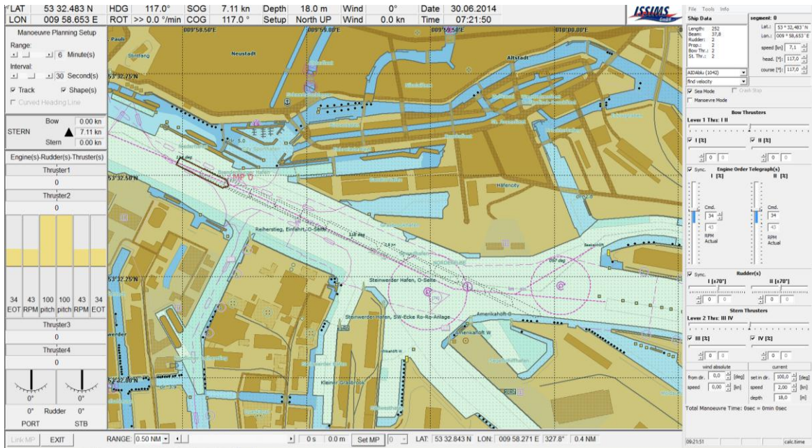
Figure 11: MP0: Initial position: The prediction already shows that the ship would drift slightly to portside due to the set handle positions.
