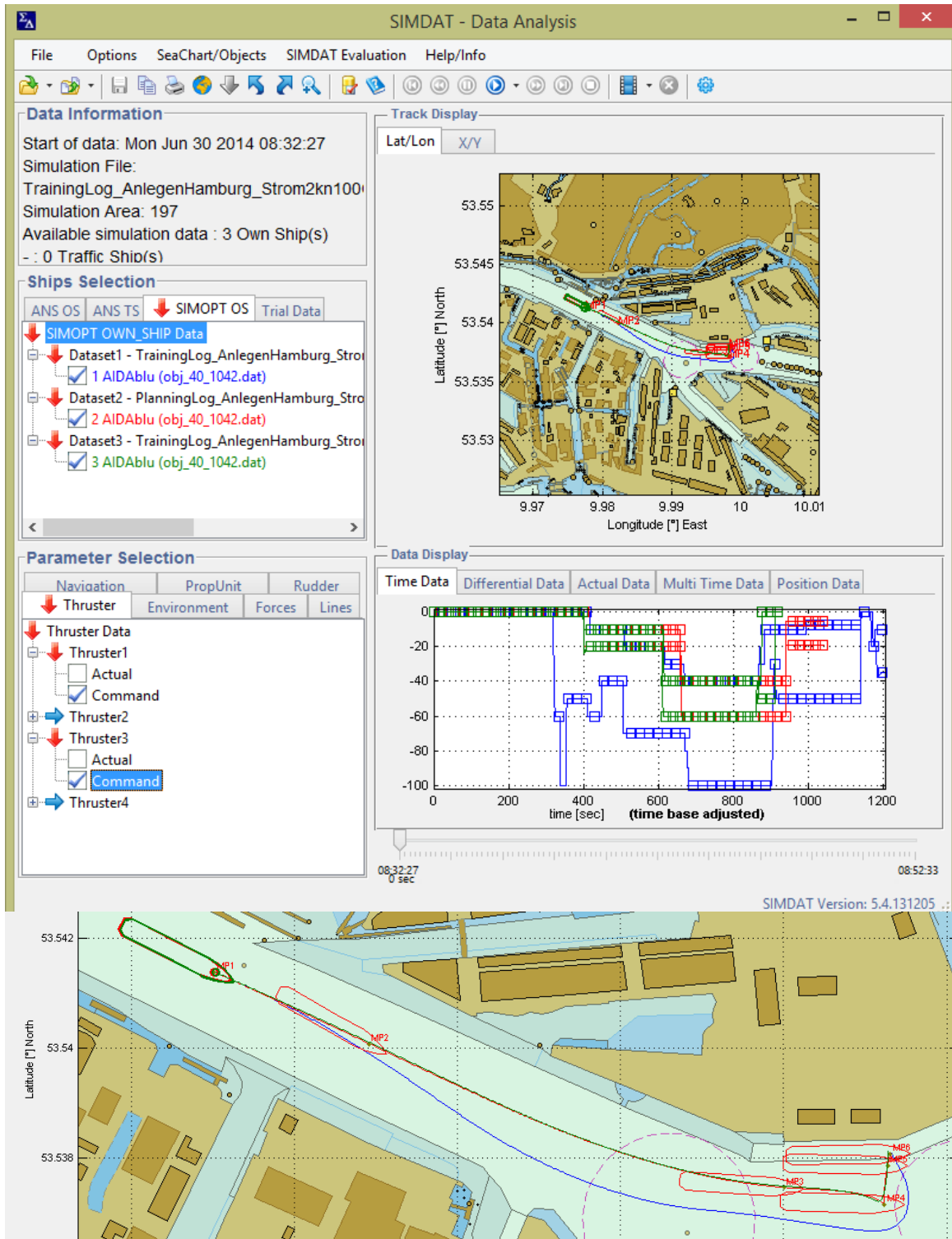
Figure 18: Results from two manoeuvring exercises in SIMDAT interface: “Track Display” with contours (Top and extract below ) and „Data Display” for time history for thruster activities
