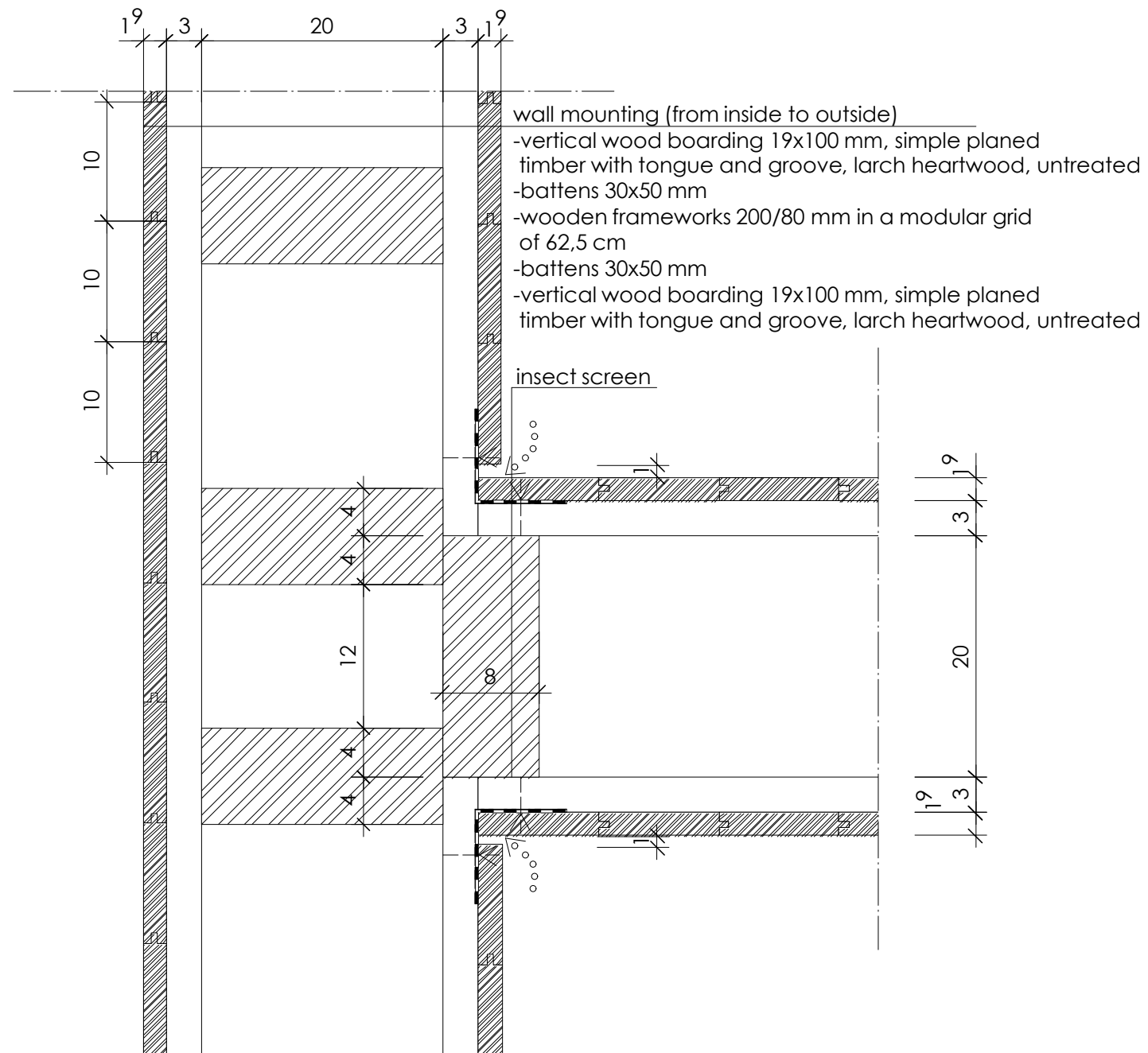
detail g1 plan of wall
