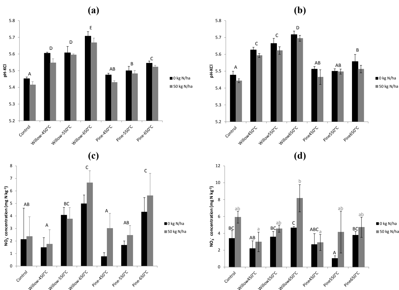
Figure 3. (a,b) pH-KCl and (c,d) \text{NO}_3^- concentrations in the control and biochar-amended treatments at two fertilizer doses (0 and 50 kg N ha -1 ) at the end of the ILVO pot trial with radish (a,c) and spring barley (b,d); error bars indicate \pm 1 standard deviation ( n = 4 ); treatments with different letters differ significantly ( P < 0.05 ) according to a Scheffé-test. In case of no interaction between the factors biochar type and fertilizer dose, there is only one letter per biochar treatment (a,b,c); in case of interaction, there is one letter on top of each bar (d) (capital and lowercase letters for unfertilized treatments and fertilized treatments, respectively).
